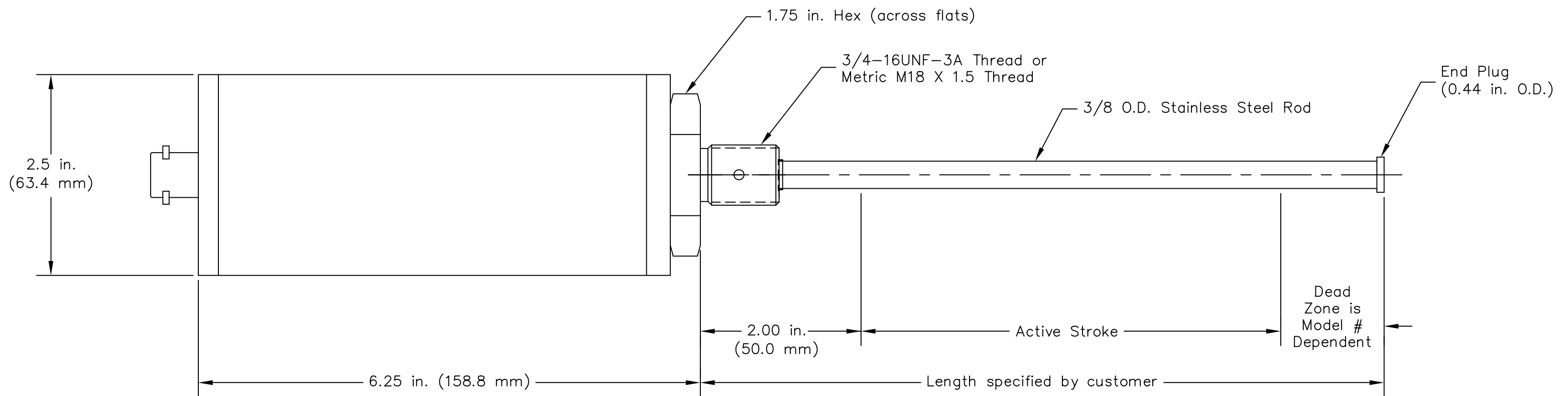
Tempo I Ruggedized Enclosures (Styles '2' & '3')
