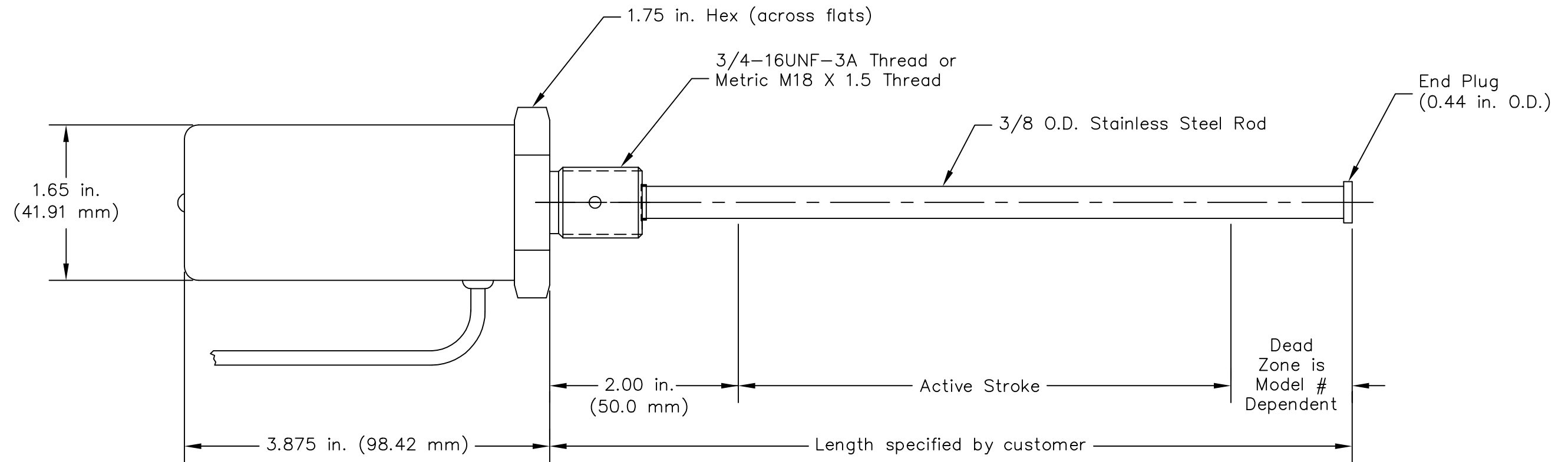
Tempo I Standard Enclosure (Style '1')
