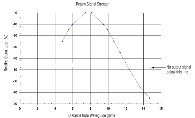
Figure 9. Temposonics C-Series - Special Considerations
