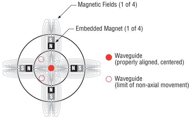
Figure 3. Bar Magnets Molded in Plastic
