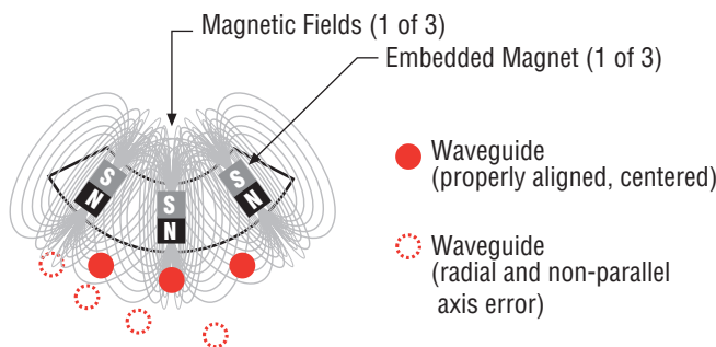
Figure 7. Bar or Button Magnet Alignment Consideration for Error Control
