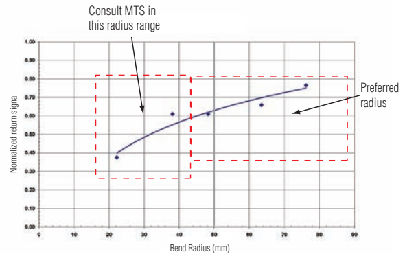
Figure 12. Sensor Path Curved to 180 degrees at Indicated Radius
