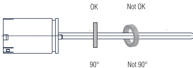
Figure 4. Keep Ring Magnet's Plane Orthogonal to the Sensor Tube Waveguide
