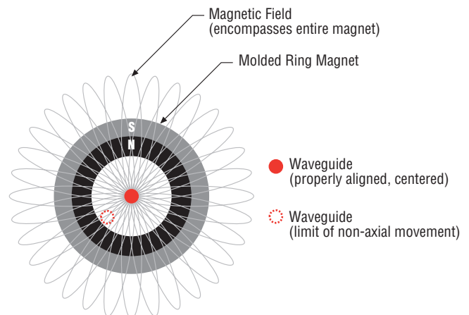
Figure 2. Molded Ferrite Ring Magnet
