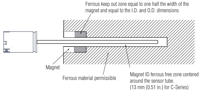
Figure 5. Ferrous Materials 'Keep Out' Area
