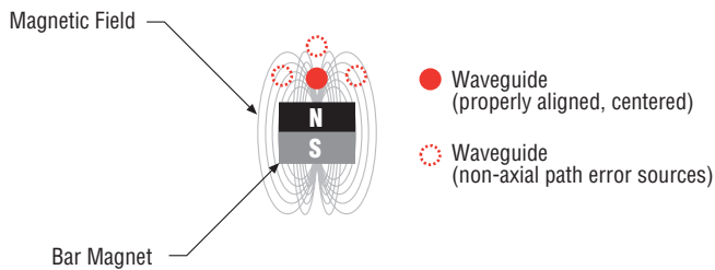
Figure 7. Bar or Button Magnet Alignment Consideration for Error Control
