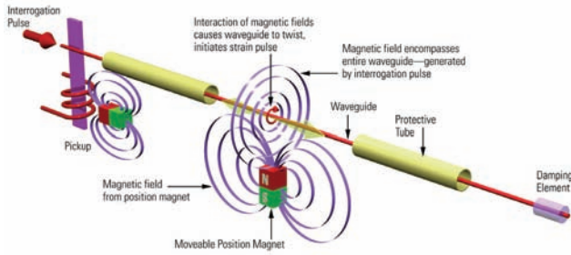
Figure 6. Single Sided Magnet Field
