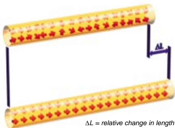
(Fig. 1) The magnetostrictive effect ( \Delta L ) is due to the orientation of Weiß areas by the influence of an external parallel magnet.
