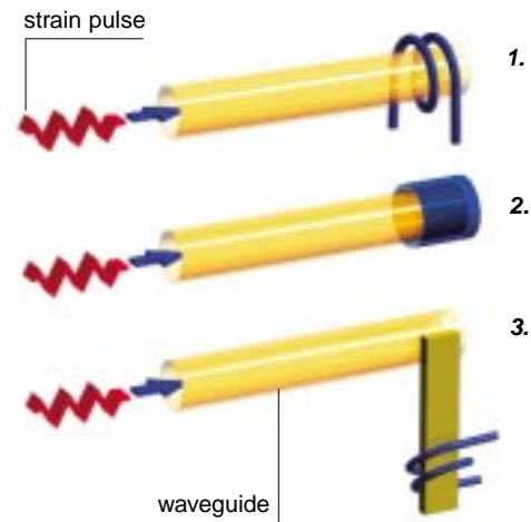
(Fig. 4) Comparison of strain pulse converter systems
