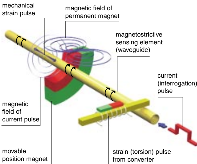
(Fig. 3) Set-up principle of magnetostrictive measurement with a Temposonics sensor comprising the following components: electronics, waveguide, position-determining permanent magnet and strain pulse converter
