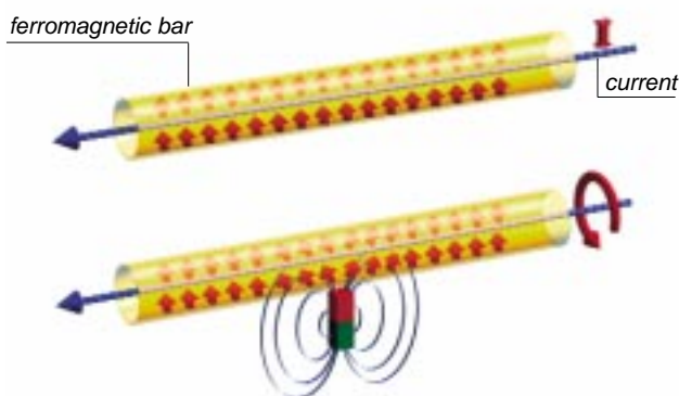
(Fig. 2) Due to the interaction of two magnetic fields, the Wiedemann effect causes mechanical distortion of a ferromagnetic bar in which an electric current flow is present.
