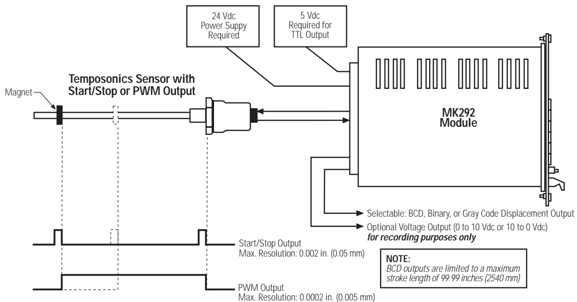
Figure 1-3 Typical System Configuration
