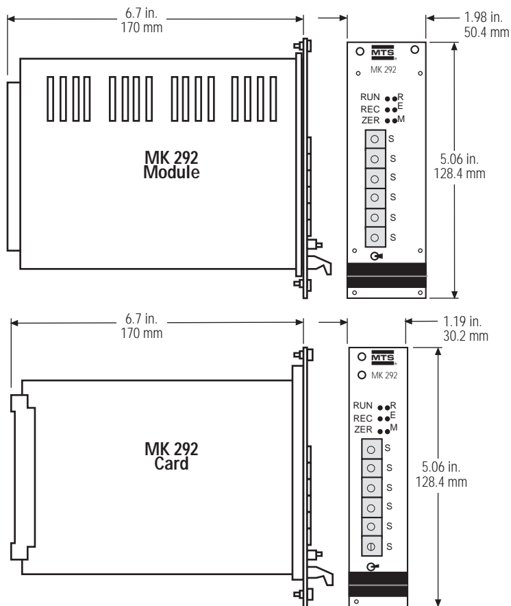
Figure 1-2 MK292 Digital Output Module Dimensions
