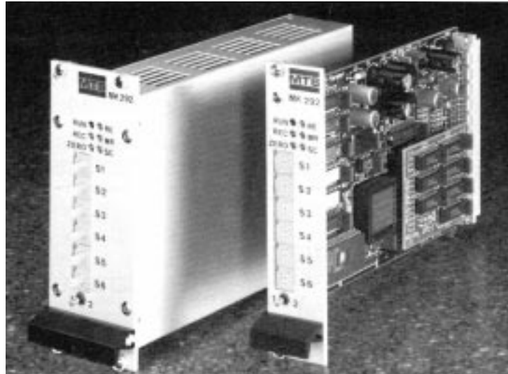
Figure 1-1 MK292 (Module version, left; card version, right)
